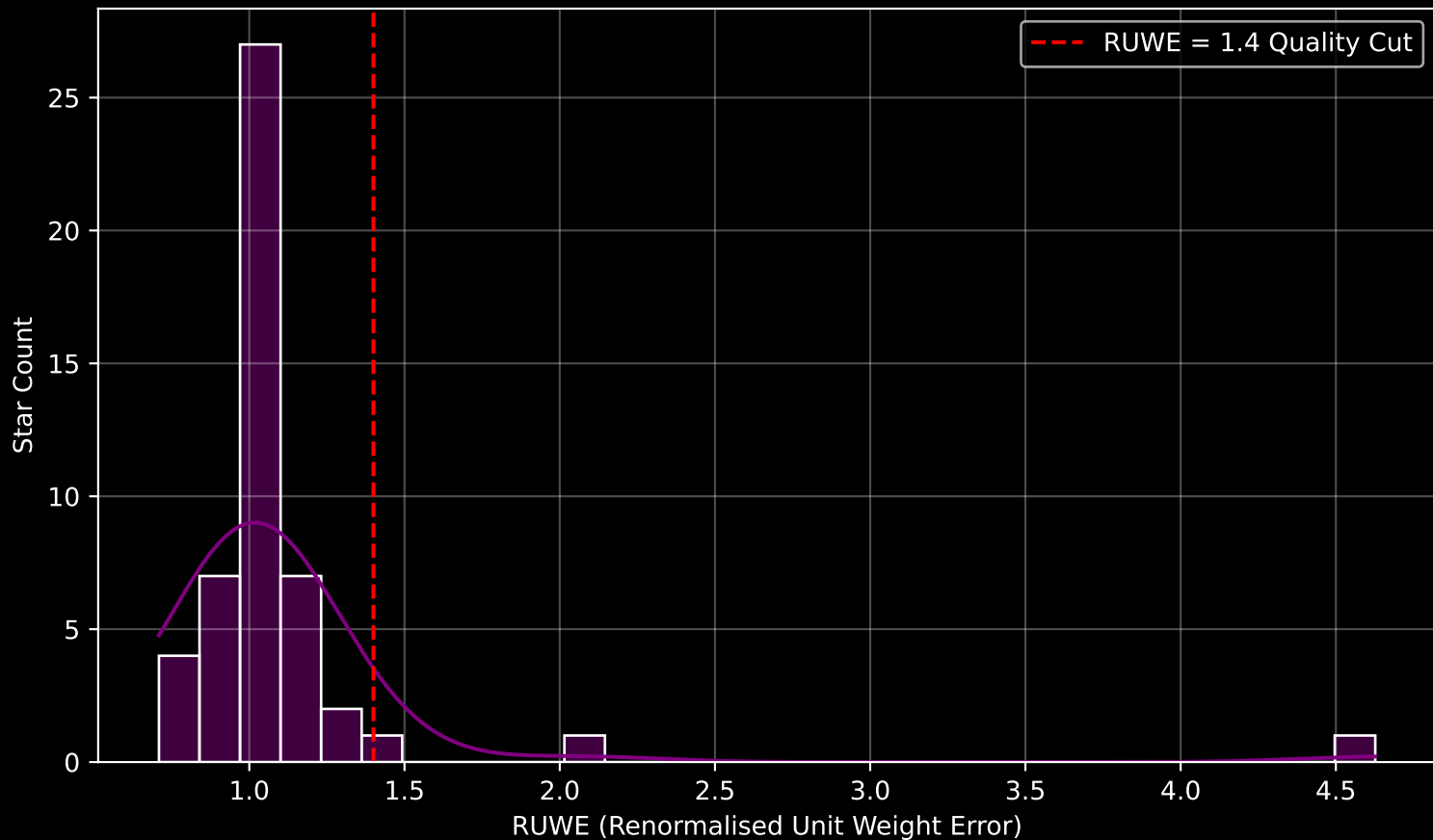
GAPOGEE DR17 Field [283-34-O] RUWE Distribution (n= 50)
