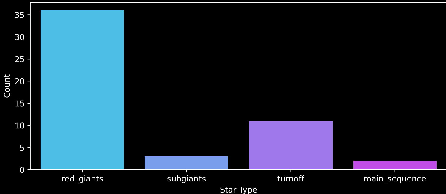
APOGEE DR17 Field: [283-34-O] Count plot of Star Type
