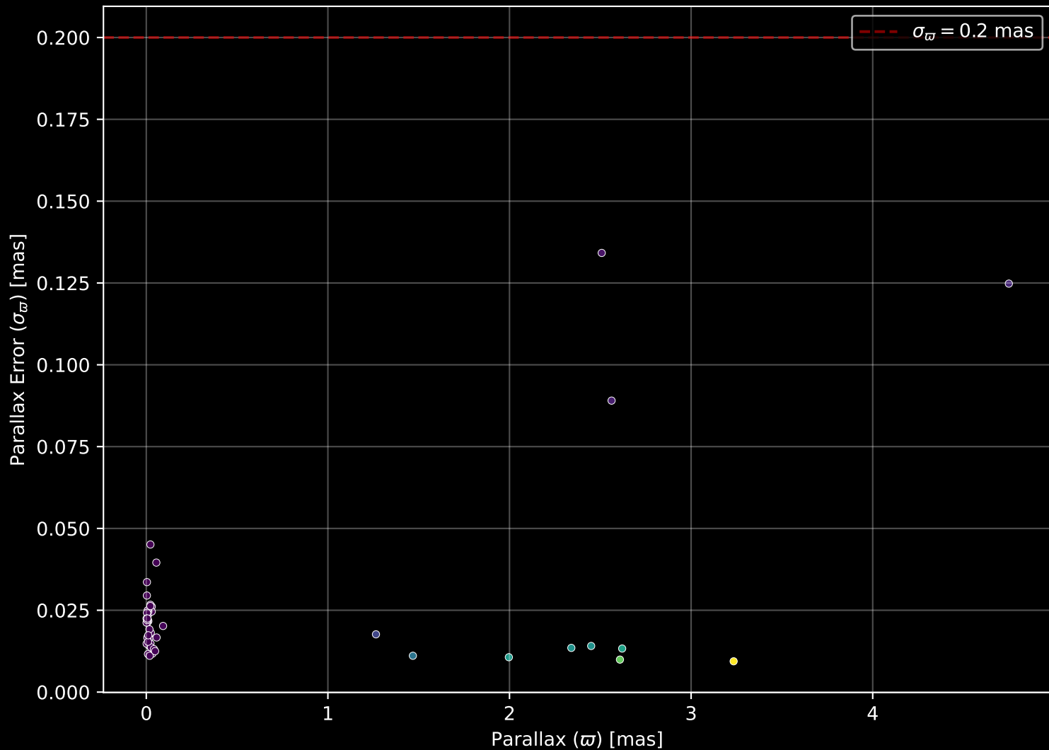
APOGEE DR17 Field: [283-34-O] Parallax Quality (n= 52)
